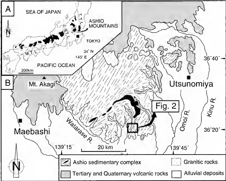
FIG. 1. — Index map showing A, the distribution of Inner Zone of southwest Japan; B, the outline of geology of the Ashio Mountains; M.T.L., Median Tectonic Line; I-S.T.L., Itoigawa-Shizuoka Tectonic Line; T.T.L., Tanakura Tectonic Line.
